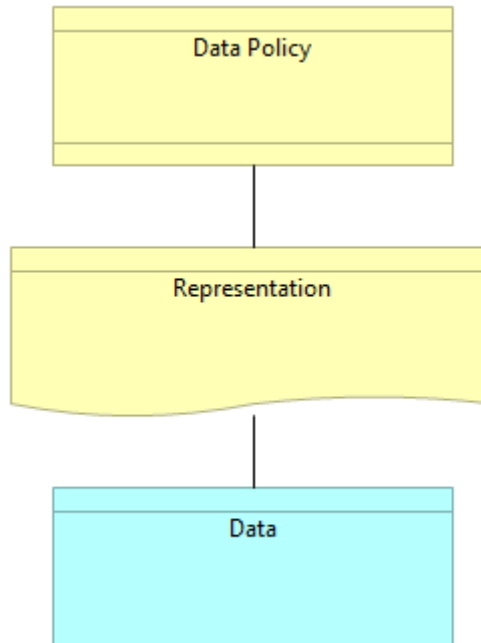
Figure 5 Semantic view
